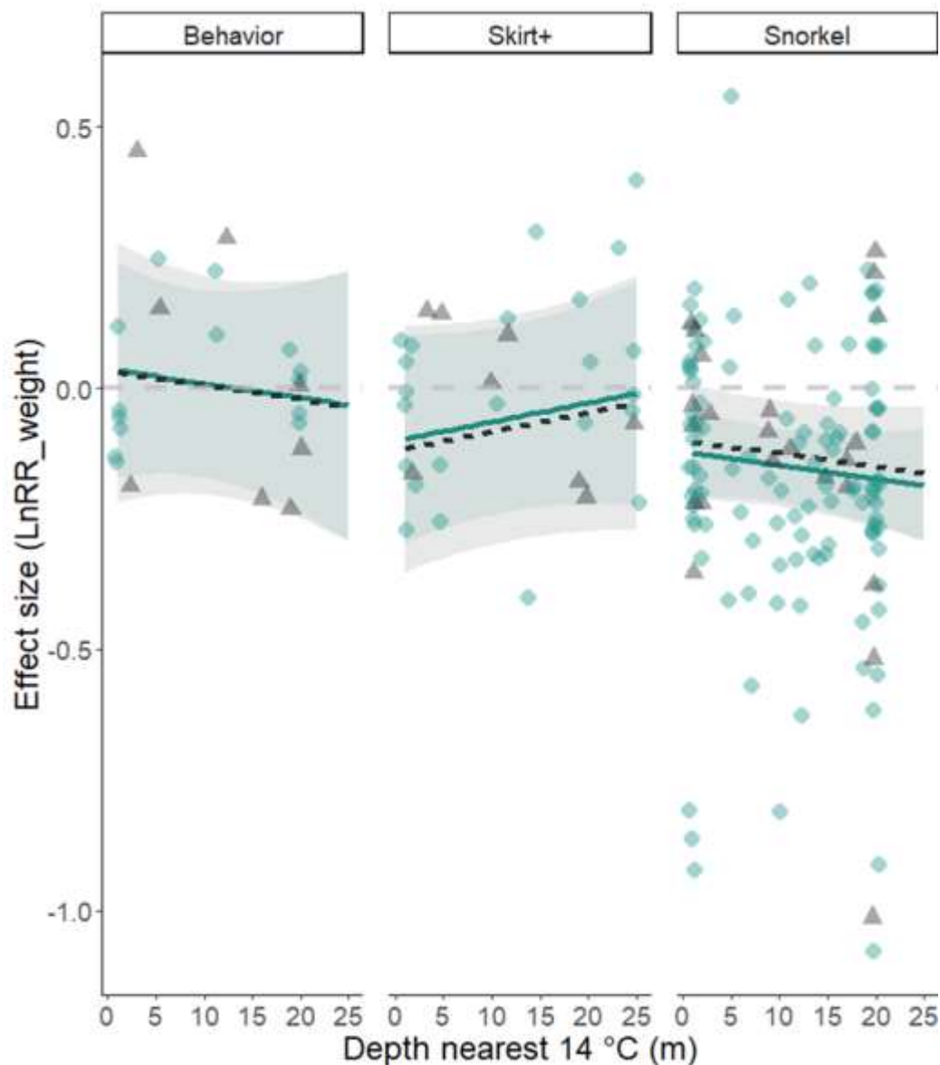
Figure 4. Influence of temperature and salinity on fish weight when using preventive tools. Effect size (natural log of the response ratio: LnRR) of fish weight as influenced by halocline (presence/absence), the depth of temperatures nearest 14 °C and preventive strategy. Solid lines and shaded areas display a fitted GLMM with 95% confidence intervals, while dot points represent each individual comparison. Green indicates no halocline, while grey indicates a halocline was present. LnRR = 0 corresponds to no difference between control and test groups while negative values indicate smaller fish in test cages.
