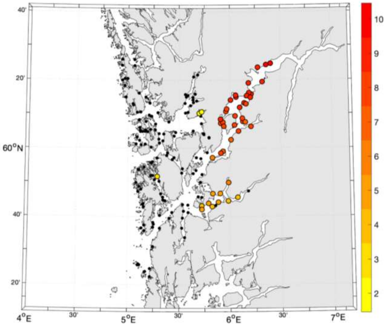
Figure 24: The depth (m) of maximum exposure to infective salmon lice copepods during the period from January 2020 to November 2022. Colored circles identify sites where the depth is between 2m (yellow) and 10m (red). Locations where the maximum was found at 1m are marked with black dots.
