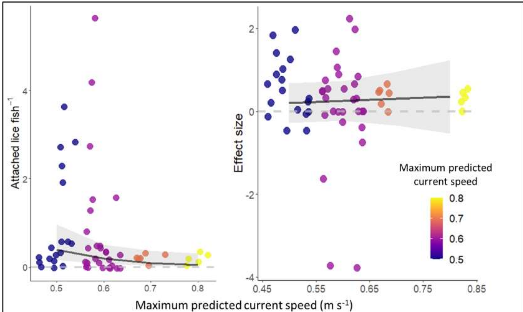
Figure 13: Influence of current speed on lice preventive efficacy. Plot (a) shows the average number of attached lice fish -1 (copepodid + chalimus 1 + chalimus 2), while plot (b) shows the standardized mean difference between observed louse attachment and predicted infestation pressure (effect size). Faded points indicate the values of each individual sampling, while solid lines and shaded areas display the fitted GLMMs with 95% confidence intervals.
