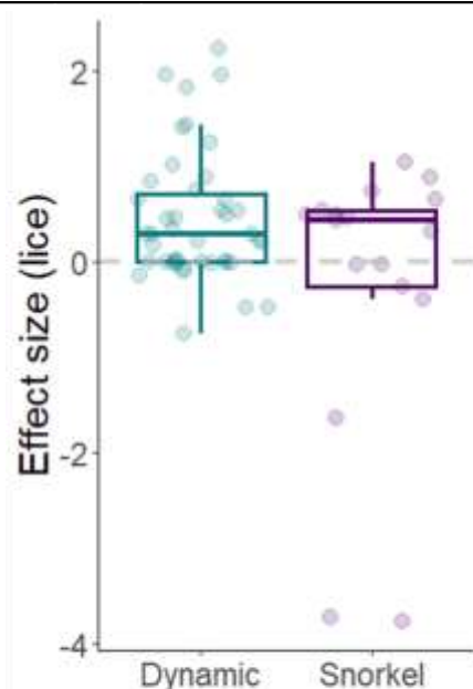
Figure 7: Boxplot showing the median and interquartile range of the standardized mean difference (effect size) between observed louse attachment and predicted infestation pressure for cages utilizing the dynamic (blue) and snorkel (purple) protection strategies.
