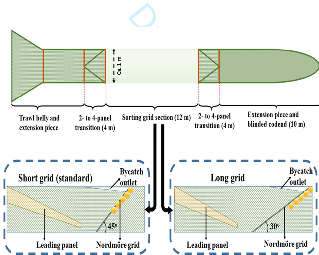
Figure 1: Illustration of the working principle of the Nordmøre grid.
