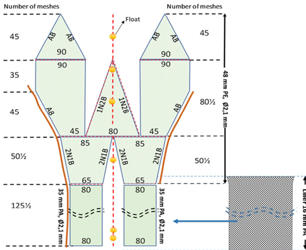
Figure 3: Technical drawing of the covers used during the experiments.
