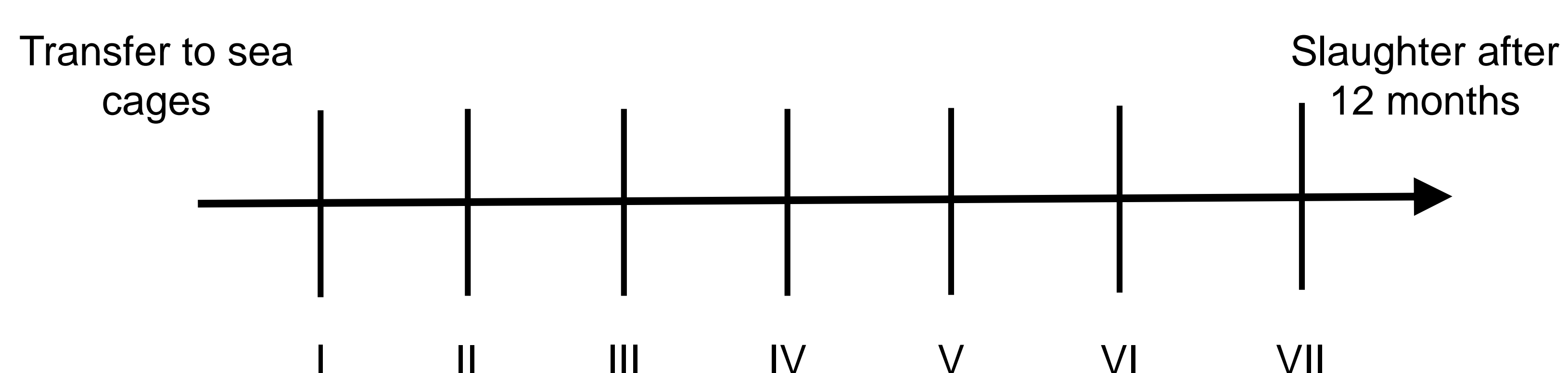
Fig. 1. Experiment outline. Large scale samplings were performed at seven different time points during the sea water phase.
