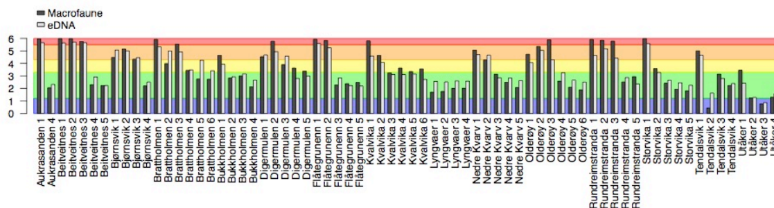
Figure 15. AMBI values inferred with morphology (black) and eDNA (white) for 70 stations from 15 farms in region Mid. As shown in the figure only 2 out of 70 stations (Olderøy 3, Brattholmen 5) are classified differently (more than 1 class) and only 2 out of 32 stations (Brattholmen 5-6) are underscored by SML from good to moderate status.
