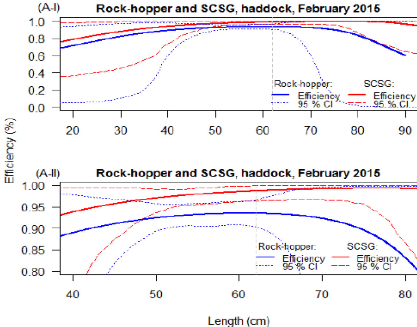
DATA ON HADDOCK: Catch efficiency for haddock for hauls with the RHG and the SCSG during February-15 (A-I). A-II show expanded area of interest.
