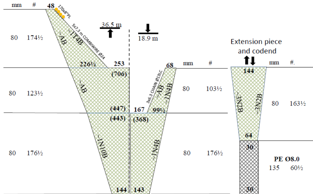
Alfredo No. 3 fish trawl – modified with 80mm Ø3,0 PE mesh in body
