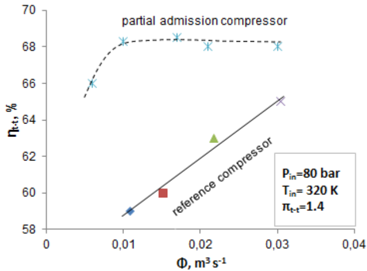
Figure 14. Prediction of overall peak efficiencies for two compressor concepts designed for different flow rates.
