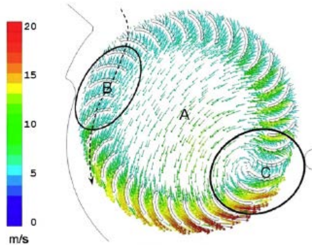
Figure 3. Three characteristic flow zones in cross flow blower. Source: Dang and Bushnell (2009)
