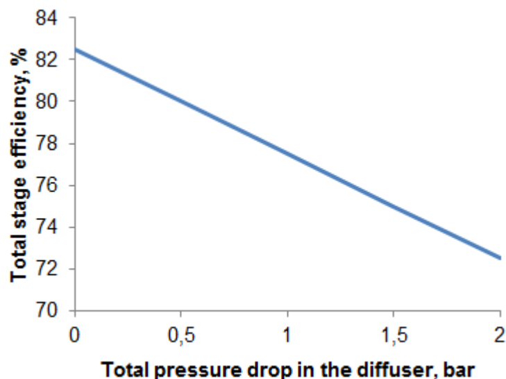
Figure 11. Stage efficiency vs diffuser total pressure drop
