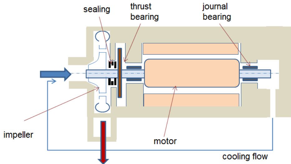
Figure 4. The reference compressor concept
