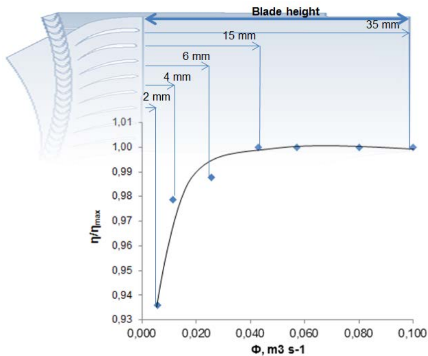
Figure 12. Predicted impact of wall effects on the performance of a partial admission compressor depending on a blade height
