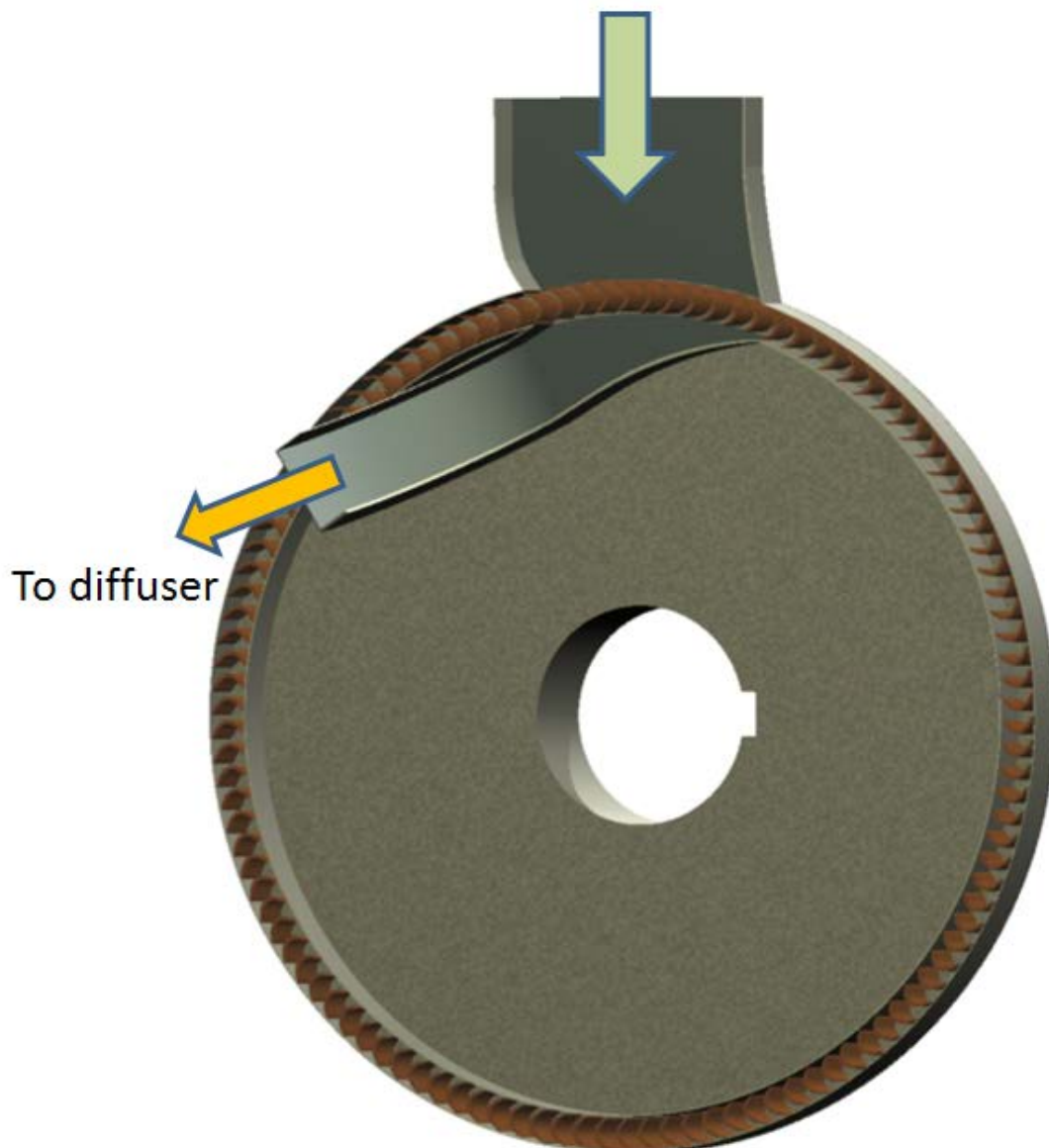
Figure 7. The concept of the partial admission CO 2 turbo-compressor
