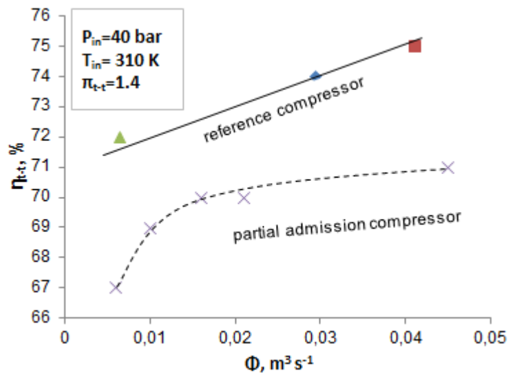
Figure 13. Prediction of overall peak efficiencies for two compressor concepts designed for different flow rates.
