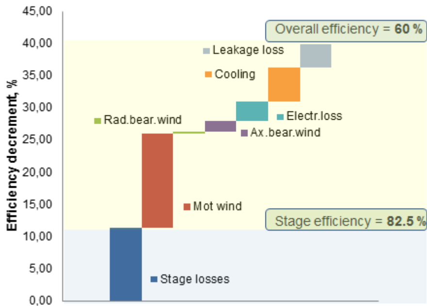
Figure 5. Predicted loss break-down for a state-of-the-art reference compressor designed for 80/113 operating pressure
