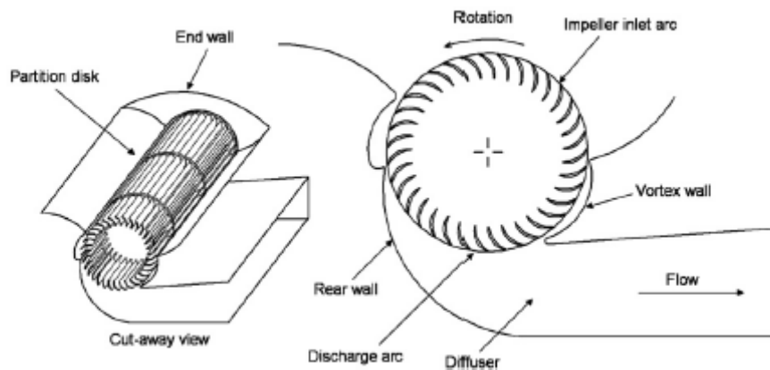
Figure 2. Typical cross-flow blower layout. Source: Dang and Bushnell (2009)
