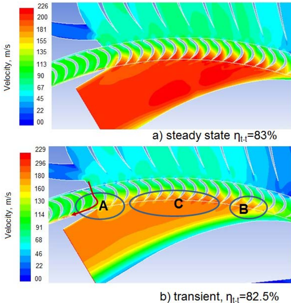
Figure 10. Comparison of velocity field obtained by steady-state and transient CFD analysis
