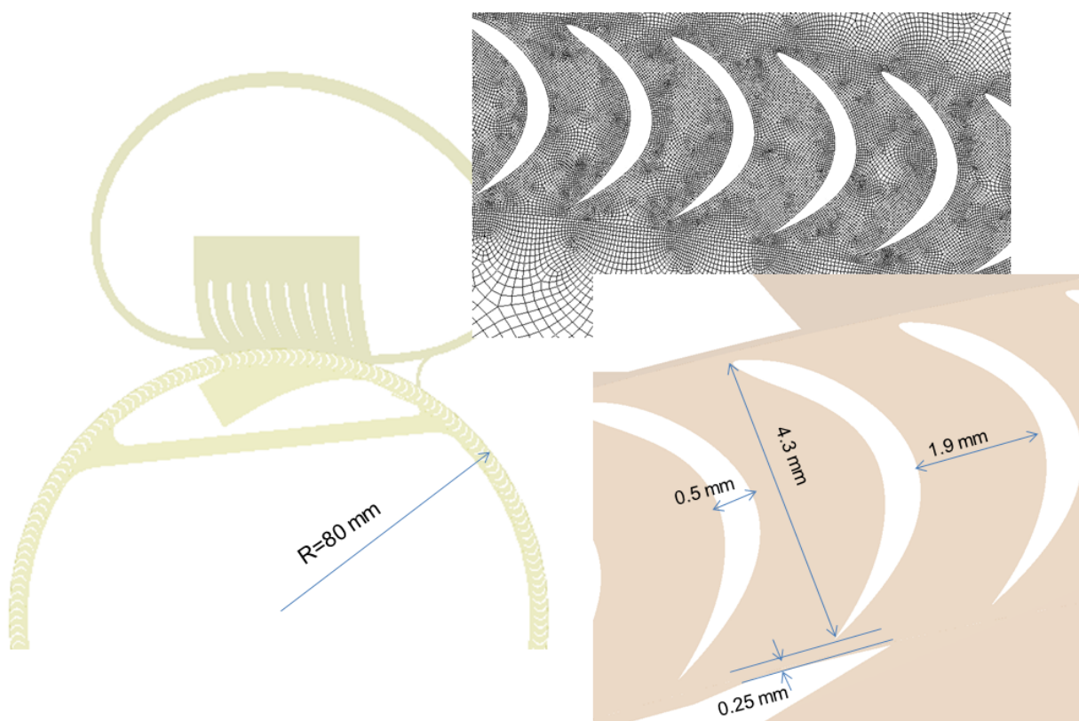
Figure 8. Two-dimensional mesh and geometry developed for steady-state and transient simulations
