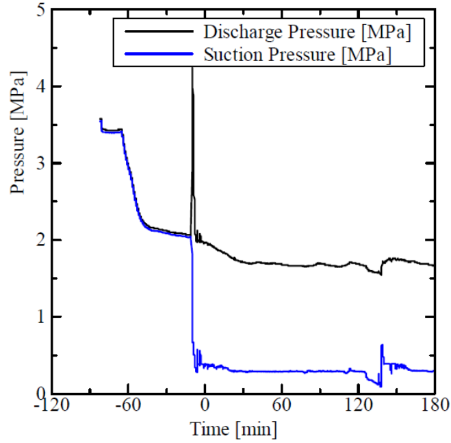
Fig 8. Measured suction and discharge pressures in LTC vary with time (the expansion valve opening in 15mm, the condensing temperature of -25°C and the heating power input 1200W).
