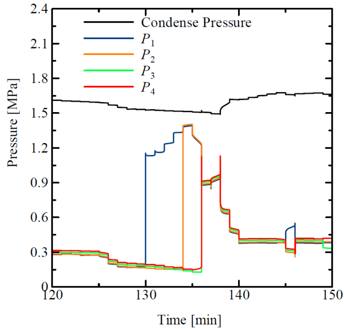
Fig 9. Behavior of measured condensing and local pressures in test section at expansion valve opening 15mm, condensing temperature -25°C and heat input 1200W
