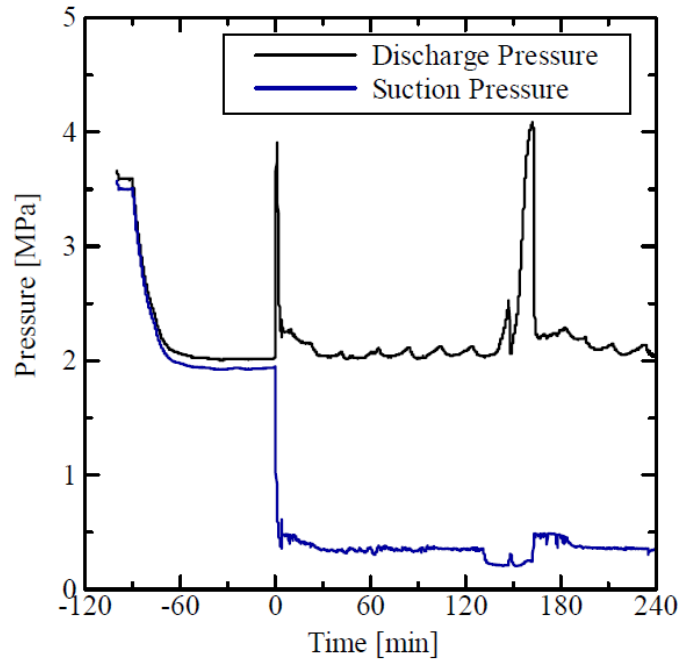
Fig 6. Measured suction and discharge pressures in LTC vary with time (the expansion valve opening in 10mm, the condensing temperature of -20°C and the heating power input 900W).
