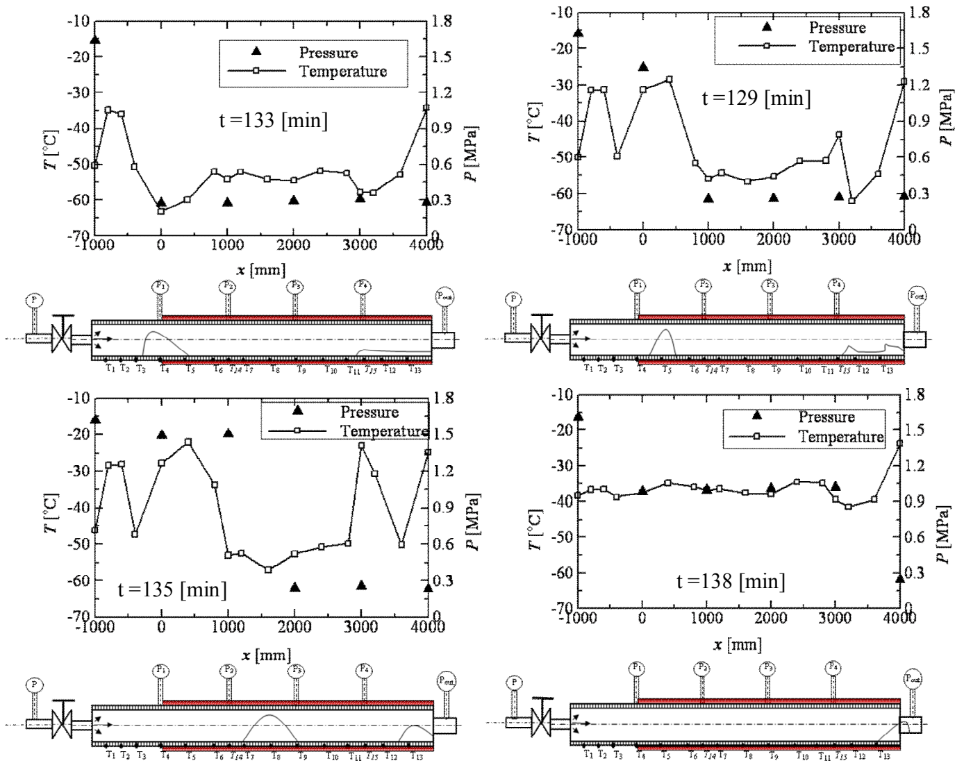
Fig. 10 Variations of local pressure and wall temperature with the dry ice sedimentation inside the test section at different times.
