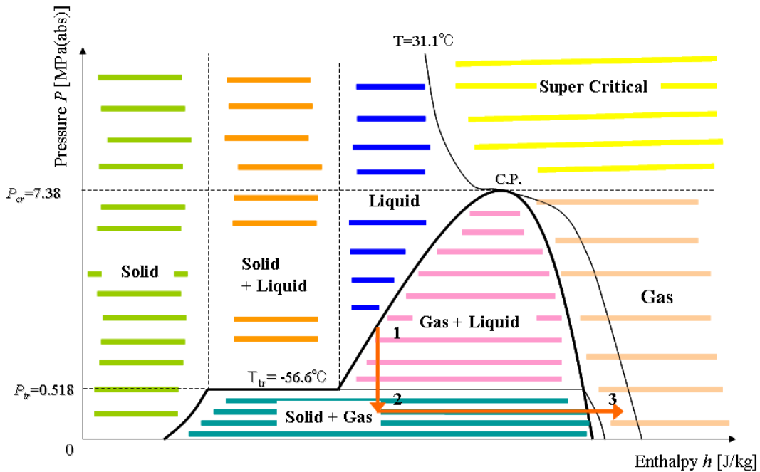
Fig 2. P-h diagram for carbon dioxide.
