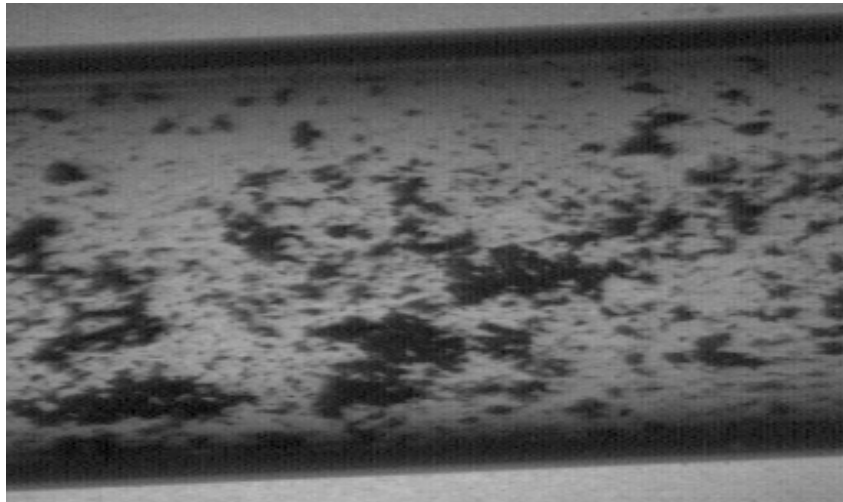
(b) CO 2 solid-gas flow at at opening conditions of 10mm of expansion valve
