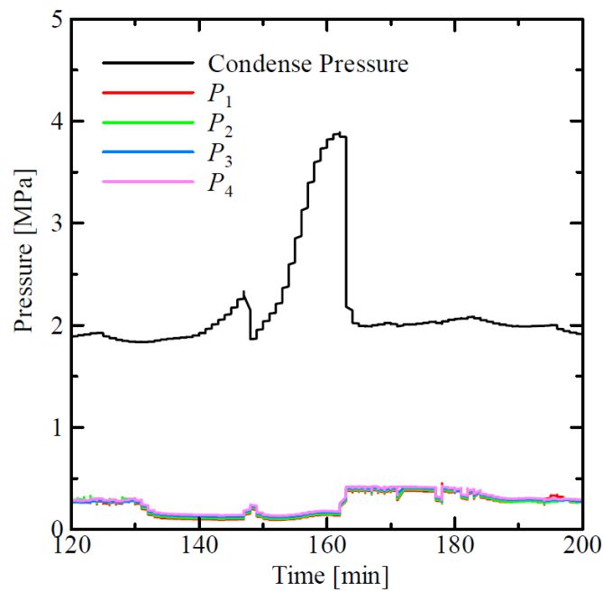
Fig 7. Behavior of measured condensing and local pressures in test section at expansion valve opening 10mm, condensing temperature -20°C and heat input 900W
