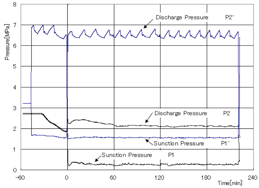
Fig 12. Variations of measured CO 2 pressures of HTC and LTC with time.
