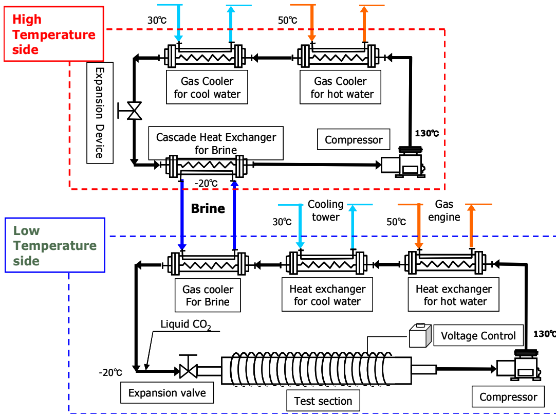
Fig 1. Schematic of the CO 2 cascade refrigeration system
