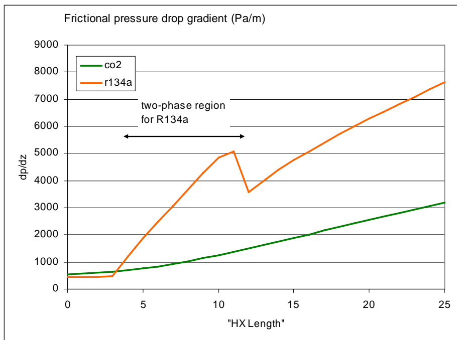
Figure 4: Frictional pressure drop for CO 2 and R134a.
