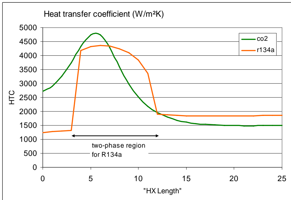
Figure 3: Heat transfer coefficient for CO 2 compared to R134a.
