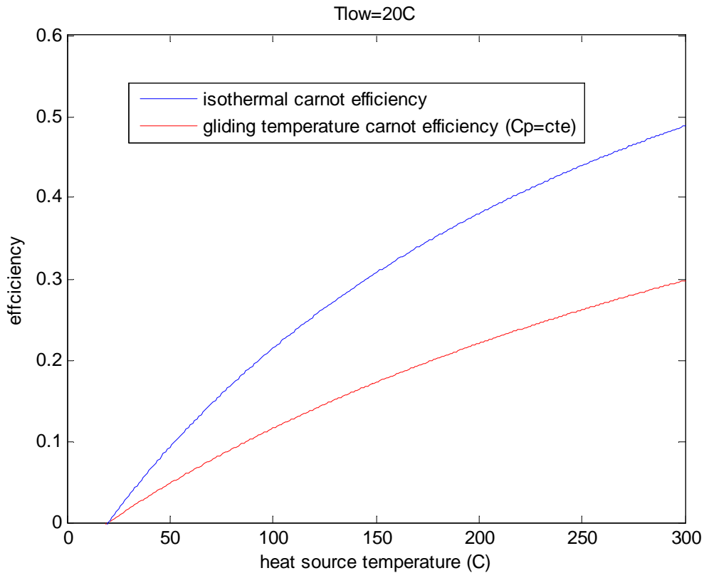
Figure 1: Maximum theoretical efficiency for constant and gliding heat source temperatures.
